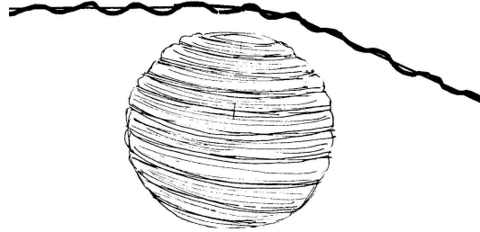
Figure 1.19. When the “bending of light” by astrophysical bodies was first measured, organized interests in Einsteinian doctrines immediately claimed such a bending to be an “experimental verification” of “Einstein’s gravitation”, and the scientific community accepted that claim without any critical inspection (for evident academic gains), according to an unreassuring trend that lasts to this day by being at the foundation of the current scientific obscurantism of potentially historical proportions. It can be seen by first year physics students that the measured bending of light is that predicted by the NEWTONIAN attraction. The representation of the same “bending of light” as being entirely due to curvature, as necessary in “Einstein’s gravitation”, implies its formulation in such a way to avoid any Newtonian contribution, with catastrophic inconsistencies in other experiments (see, e.g., next figure).
