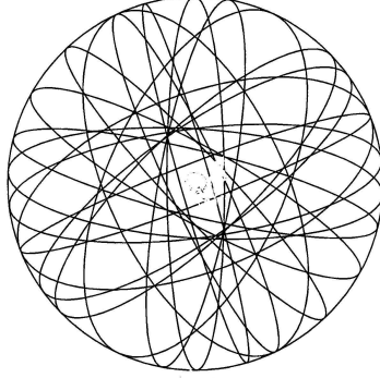
Figure 3.6. A schematic view of the “isosphere”, namely, the perfect sphere on isospace over isofield represented by isoinvariant (3.2.121), that is assumed as the geometric representation of hadrons used in this monograph. The actual nonspherical and deformable shape of hadrons is obtained by projecting the isosphere in our Euclidean space, as illustrated in the last identify of Eq. (3.2.122).
